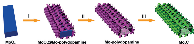
Figure 1. Schematic illustration of the formation procedure of hierarchical \beta - \text{Mo}_2\text{C} nanotubes. Stage I: growth of Mo-polydopamine hybrid nanosheets on the pre-synthesized \text{MoO}_3 nanorods. Stage II: further growth of nanosheets and simultaneous dissolution of the \text{MoO}_3 nanorods. Stage III: formation of hierarchical \beta - \text{Mo}_2\text{C} nanotubes by annealing the Mo-polydopamine nanotubes.
